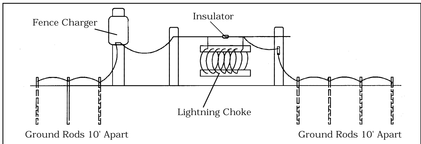
Figure 2. Grounding Procedures for Electric Fence Chargers
